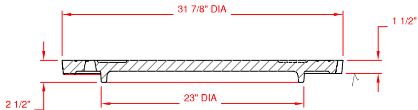
COVER SECTION
