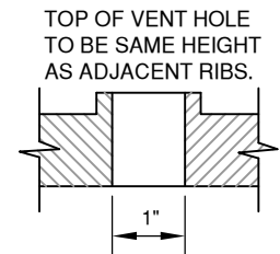
DETAIL OF VENT HOLE
