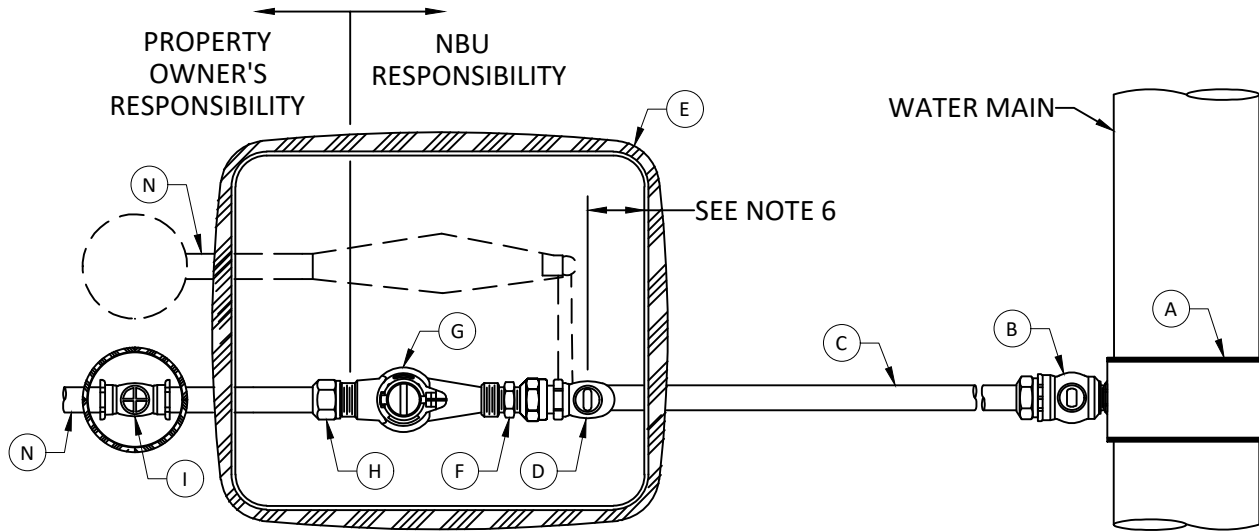
WATER SERVICE TAP PLAN VIEW
