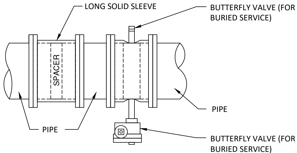
TOP VIEW
