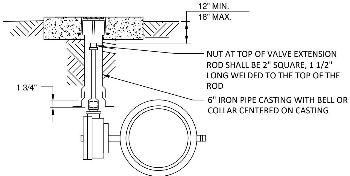
END VIEW
