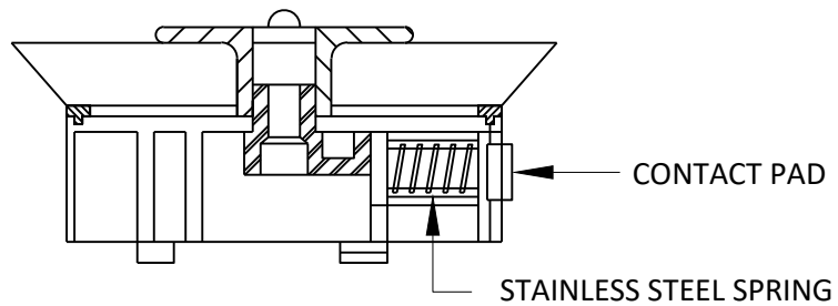
SECTION VIEW
