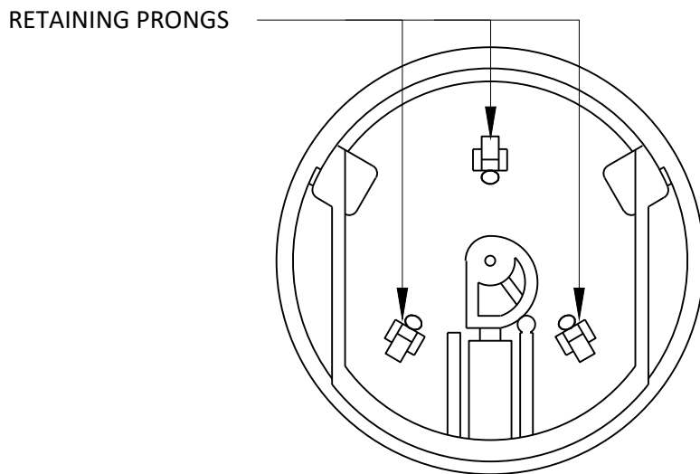
BOTTOM VIEW
