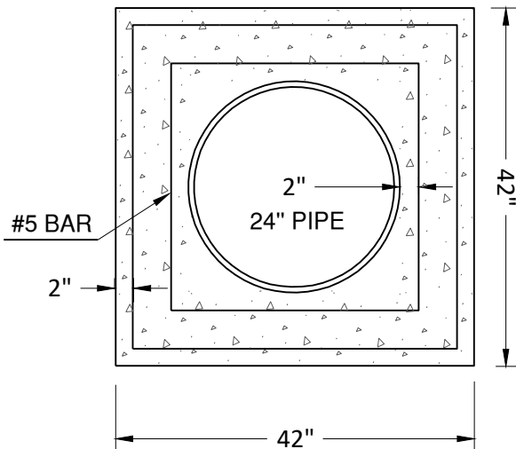
42" X 42" CONCRETE PAD
